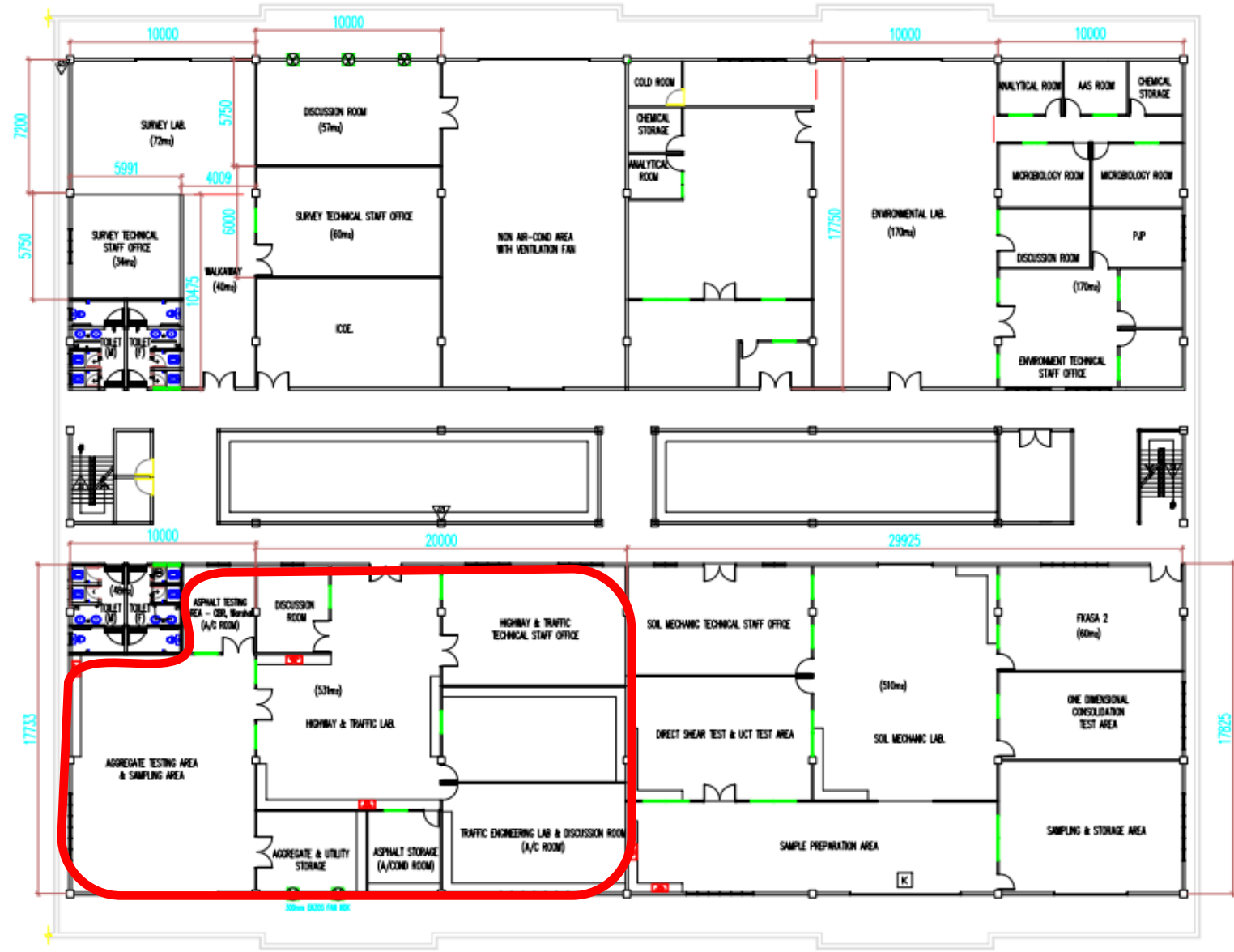
GROUND FLOOR PLAN CIVIL LAB
